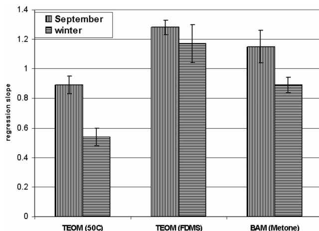
Figure 4. Regression slope between FRM (independent variable) and continuous methods under different seasons at the field site.
