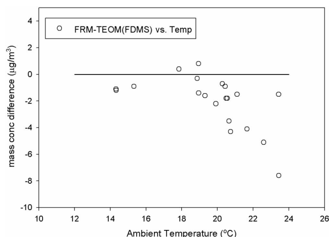
Figure 3. Difference of PM_{2.5} mass concentration measured between the FRM and TEOM (FDMS) monitor as a function of ambient temperature at field site during summer sampling campaign.
