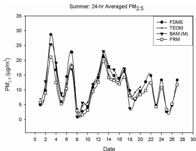
Figure 2. Time series of PM measurement made with two beta gauges, two TEOMs, and a FRM sampler at Ewing, NJ, in September 2004.
