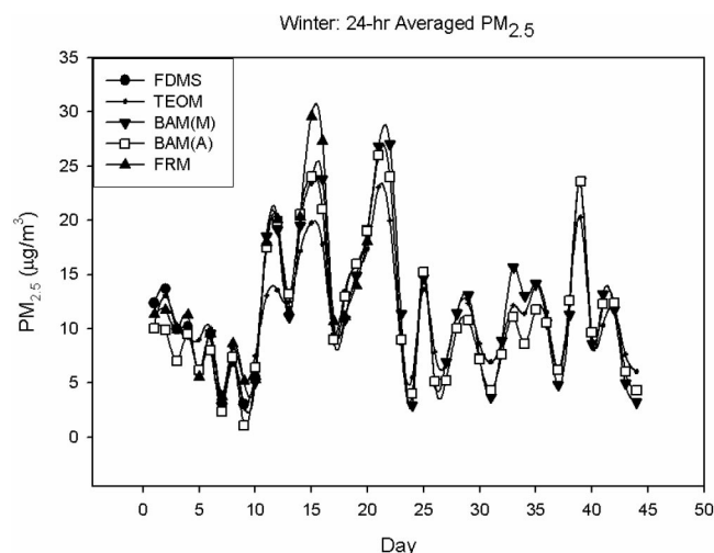
Figure 1. Time series of 24-hr integrated PM_{2.5} measurements made with two beta gauges, two TEOMs, and a FRM sampler at Ewing, NJ, between December 2004 and February 2005.
