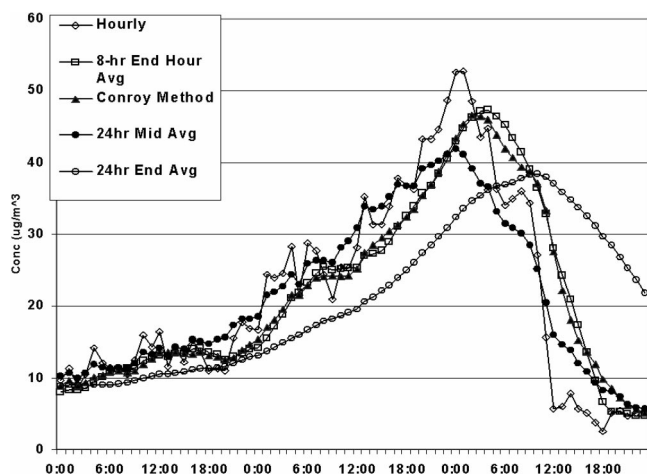
Figure 5. PM_{2.5} data from the TEOM (FDMS) monitor at Ewing, NJ for the period from 12:00 a.m. October 29, 2004 through 11:00 p.m. October 31, 2004. Reporting methods include: hourly average, 8-hr end-hour average, Conroy method, 24-hr mid-hour average, and 24-hr end-hour average.
